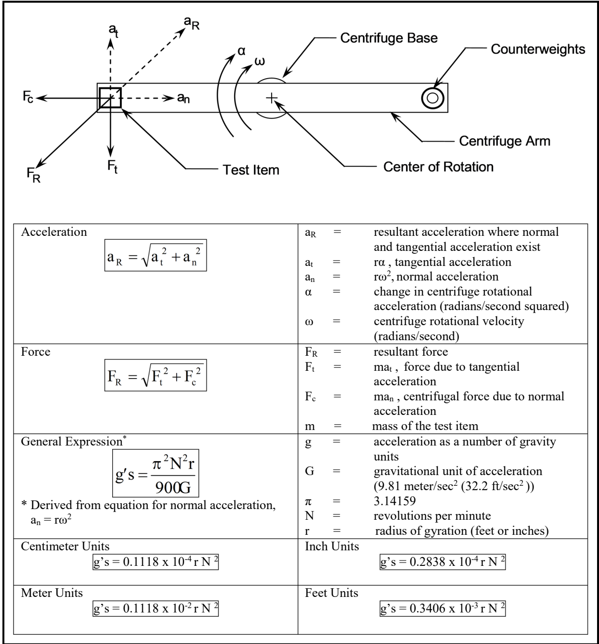
Figure 513.8A-4. Basic forces imposed on test item due to accelerations produced by centrifuge.
