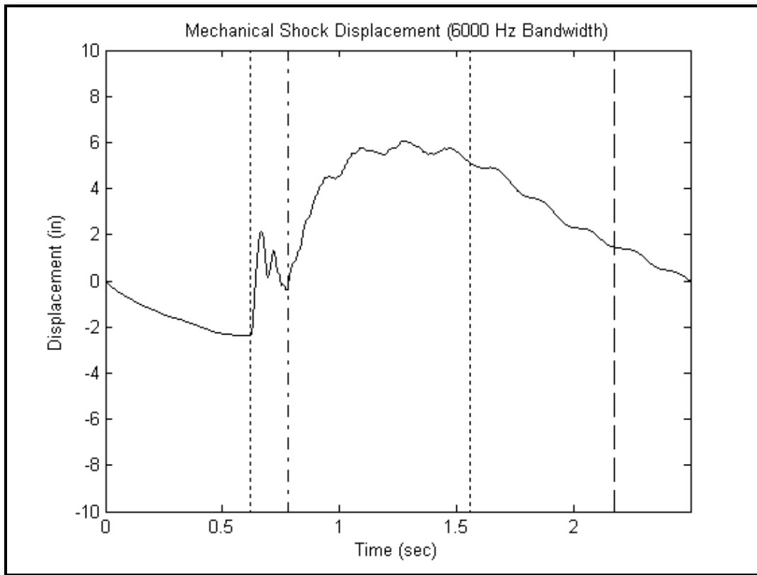
Figure 516.8B-5. Measurement displacement via integration of velocity after mean (DC) removal.
