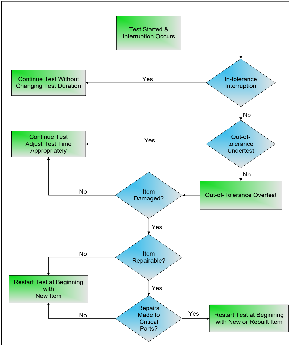
Figure 1-5. Interrupted test cycle logic.
