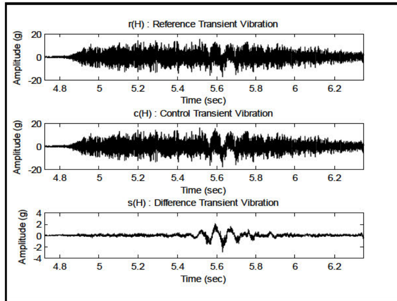
Figure 525.1A-10. Transient vibration time traces - r, c, and s.
