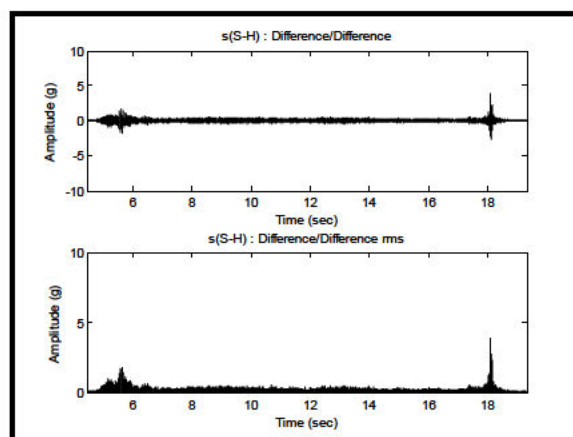
Figure 525.1A-9c. Time Trace of Difference of the Differences ((S) – (H)).
