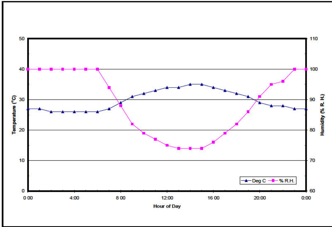
Figure 507.6-5. Natural Cycle B2 – Cyclic high humidity.
