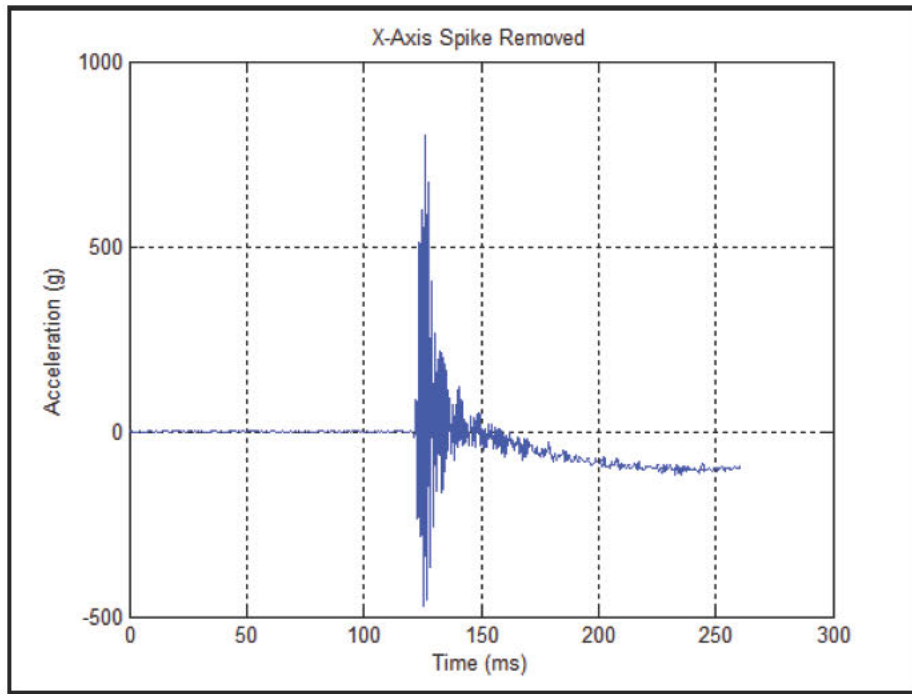
Figure 517.2A-9. Time history of wavelet correction removed from the acceleration time history in Figure 517.2A-5.
