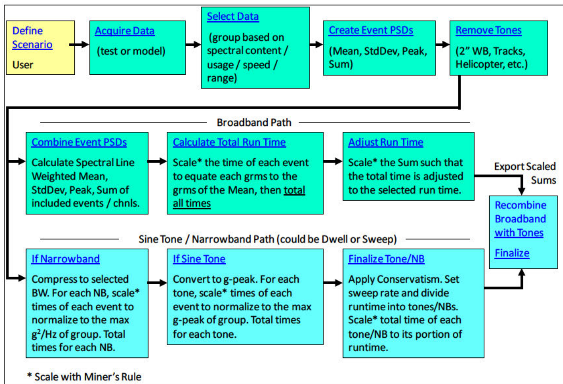
Figure 514.7F-D.1. VSD flowchart.
