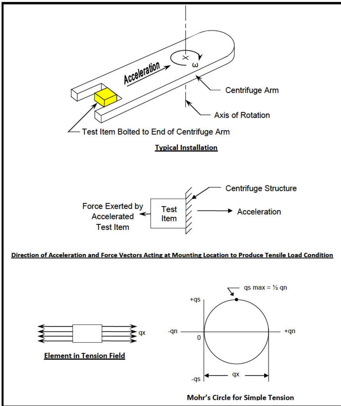
513.7A-3. Basic centrifuge test installation resulting in tensile load conditions.
