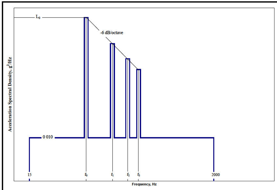
Figure 514.7D-2 – Category 13 - Propeller aircraft vibration exposure. (Same as Annex C, Figure 514.7C-8.)
