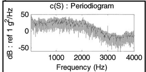
(e) Control Time Trace Slip Table (S)
