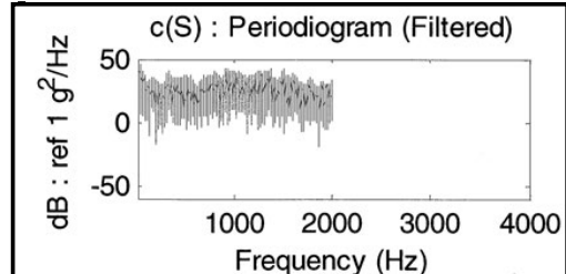
(f) Bandlimited Control Time Trace Slip Table (S) (10 Hz – 2000 Hz)
