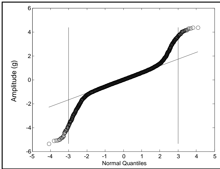
Figure 519.7B-11b. qq-plot, gunfire shock time trace difference (4000 rnd/min).
