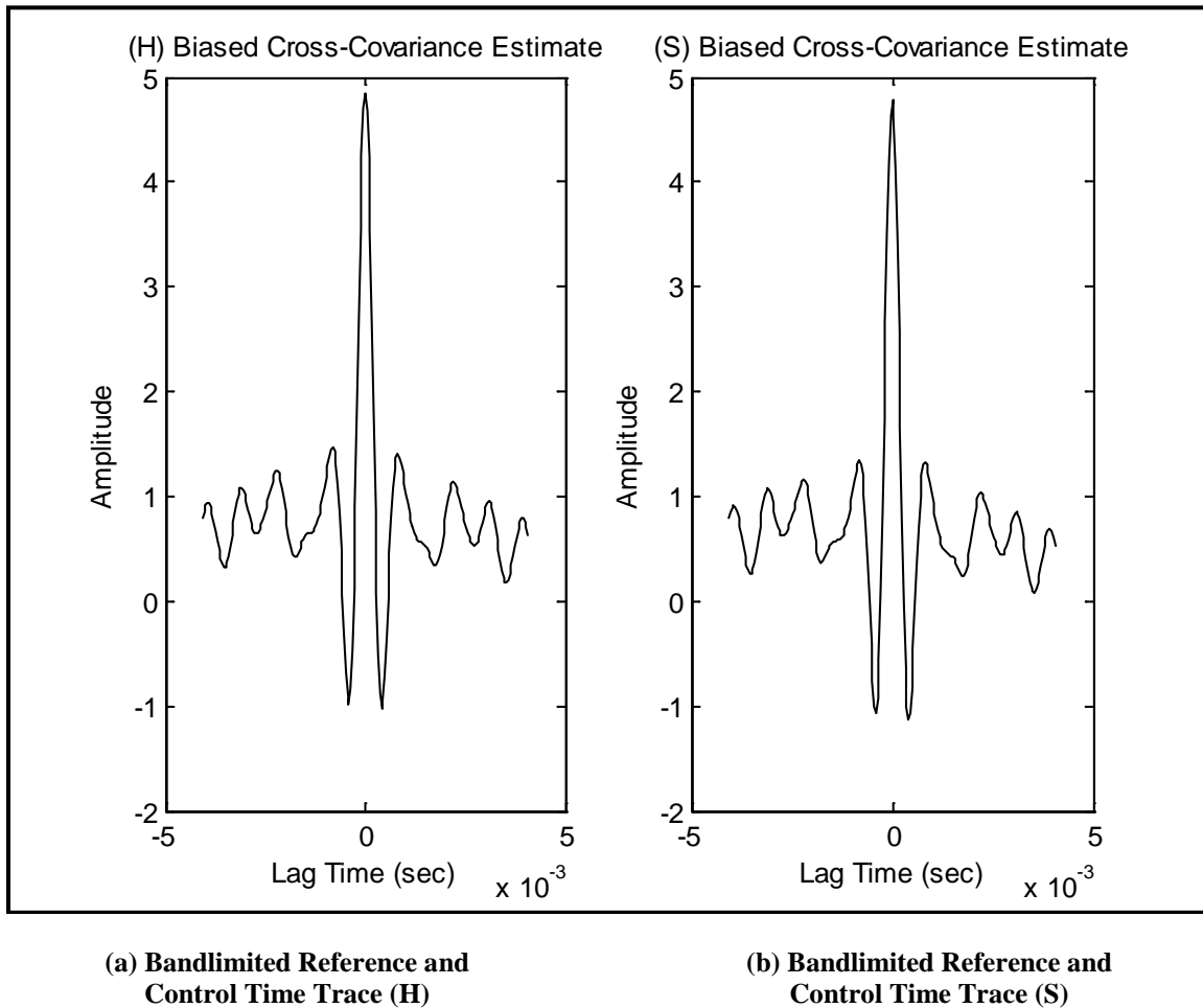
Figure 525.1A-4. Cross-covariance function estimates between reference and control time traces.
