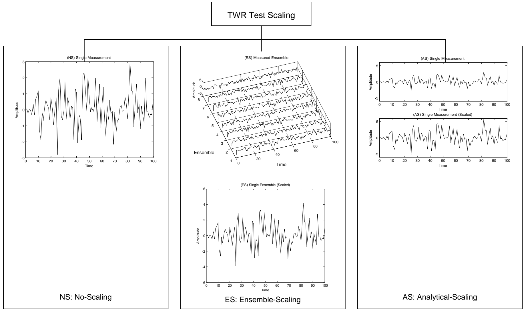
Figure 525.1-1. Basic TWR test modes as related to time trace scaling.
