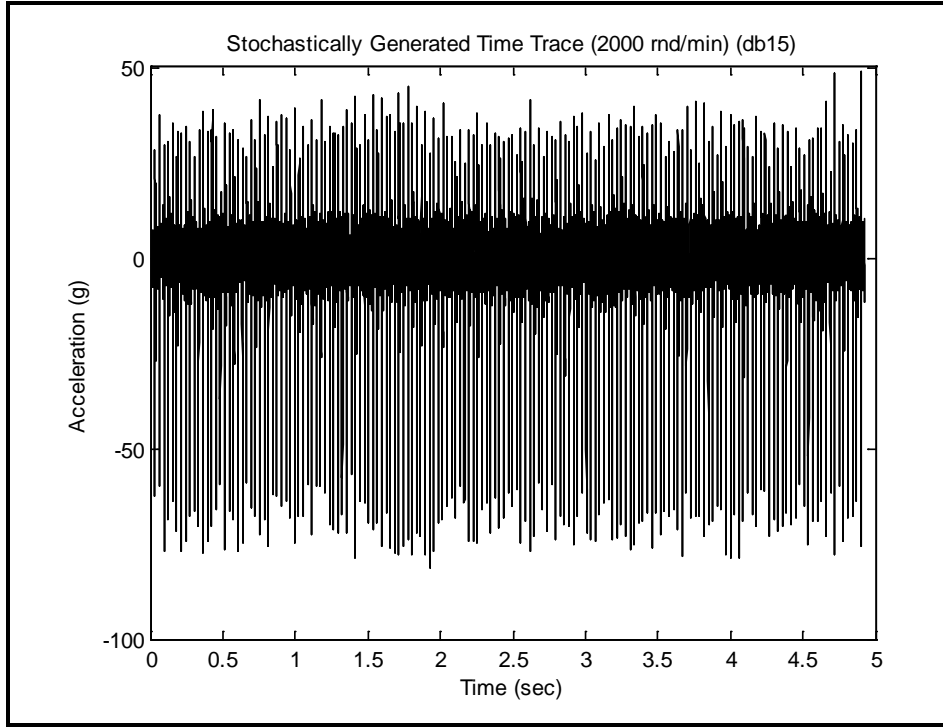
Figure 519.7B-9a. Stochastically generated gunfire shock time trace (2000 rnd/min).
