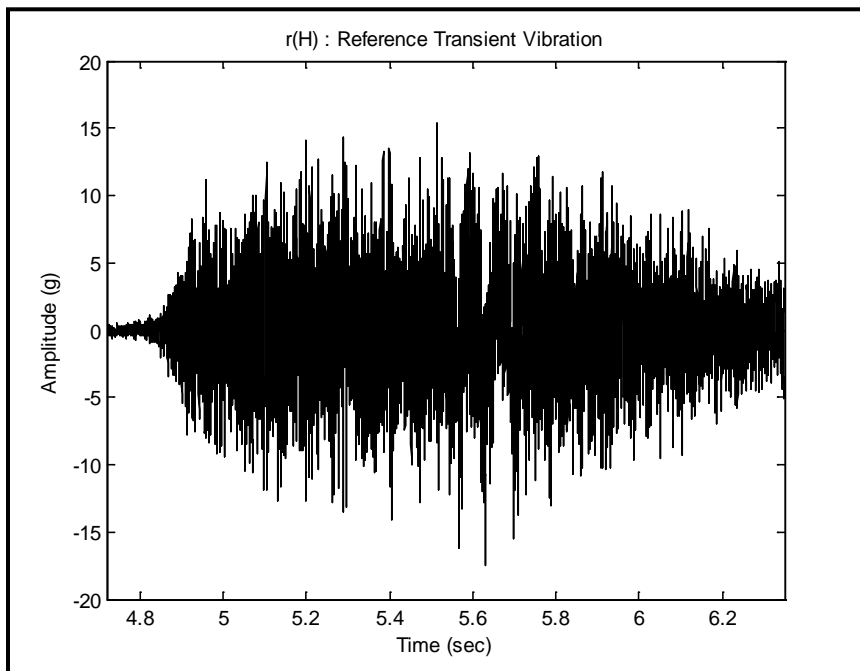
Figure 525.1A-6. Transient vibration reference time trace segment.
