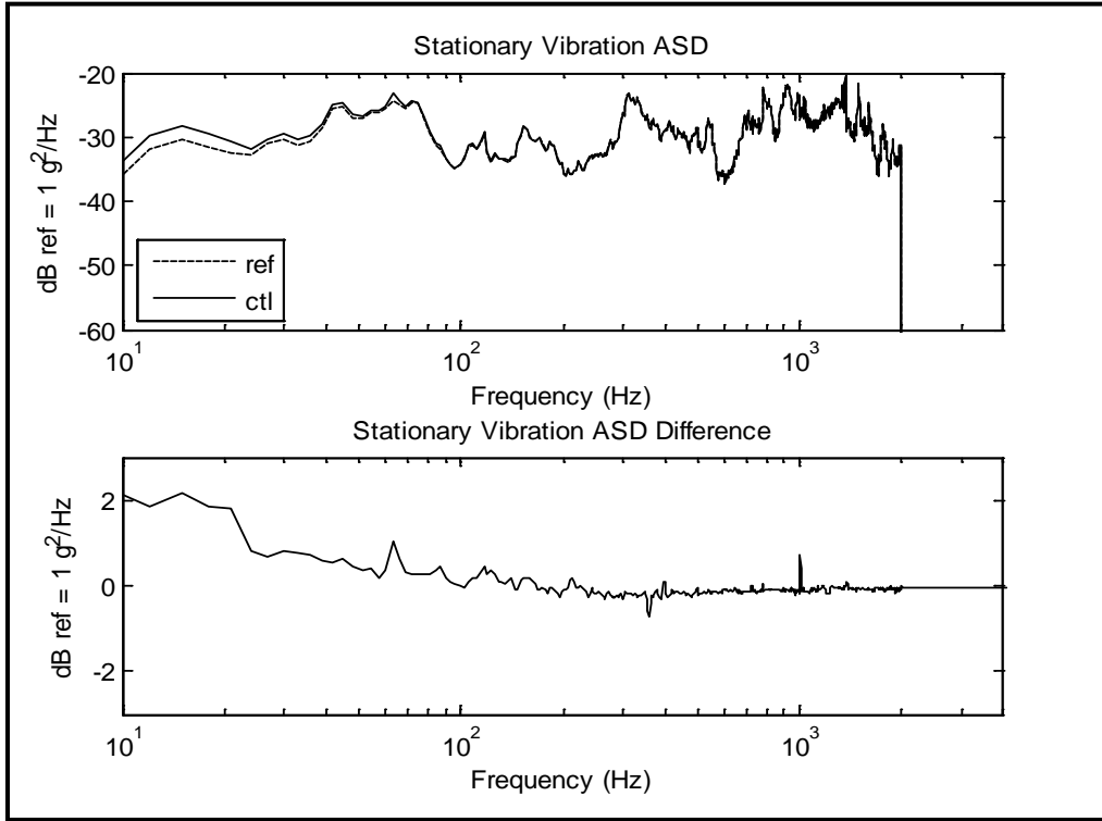
Figure 525.1A-19a. Composite ASD estimates for r and c.
