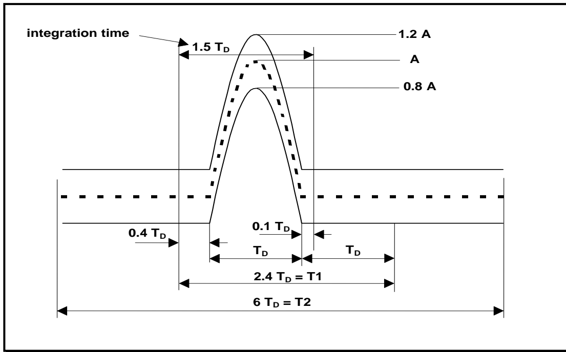
Figure 516.7-12. Half-Sine shock pulse configuration and tolerance limits (for use when reference criteria are provided as a classical half-sine pulse).
