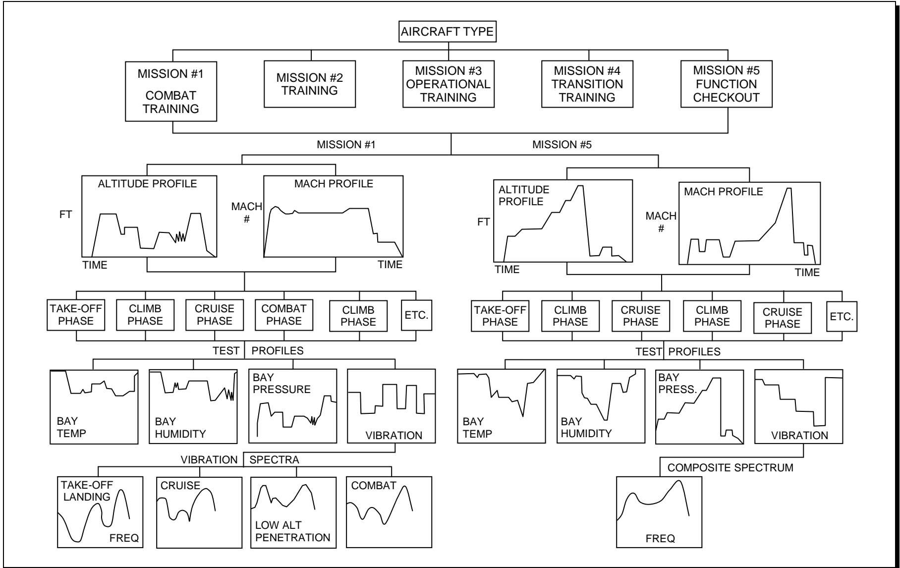
Figure 520.4-2. Test profile generation flow diagram
