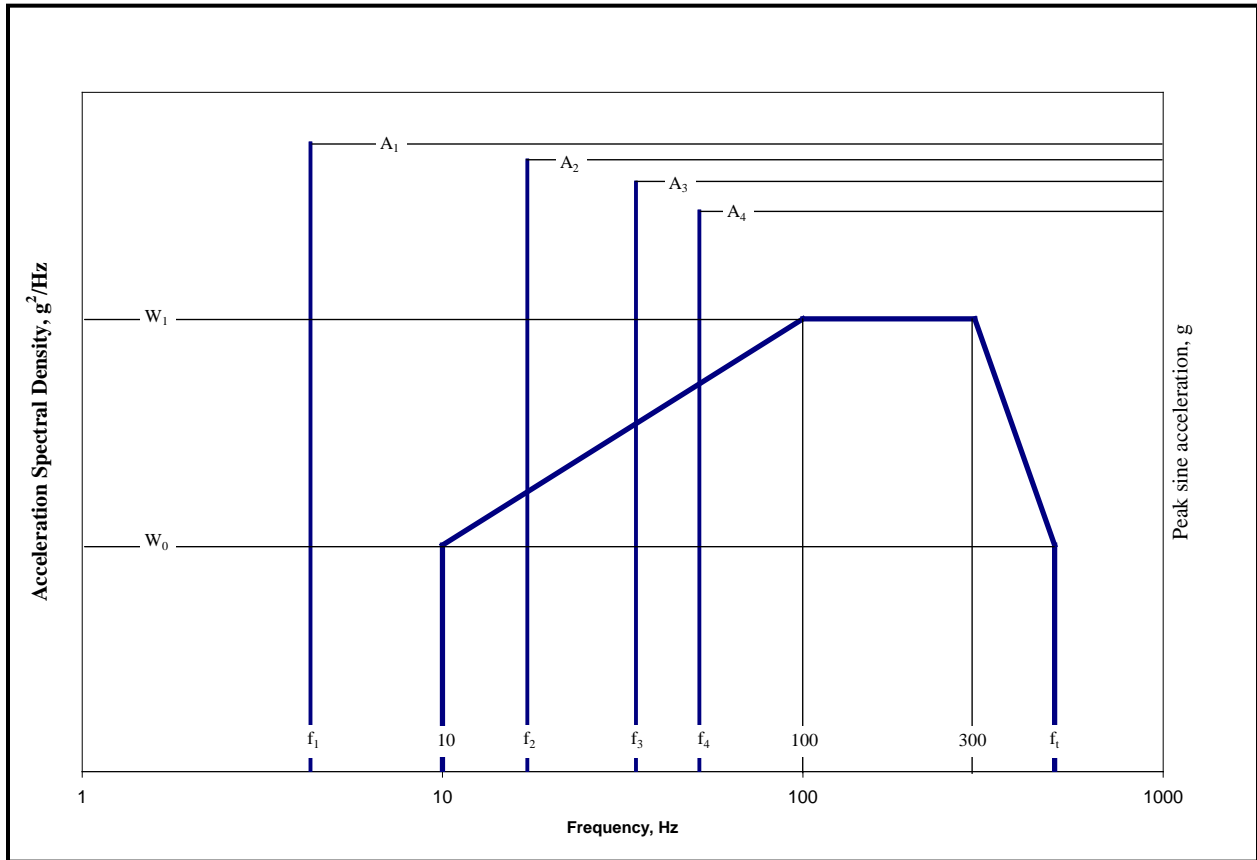
Figure 514.7D-3 Category 14 – Helicopter vibration (Same as Annex C, Figure 514.7C-9).
