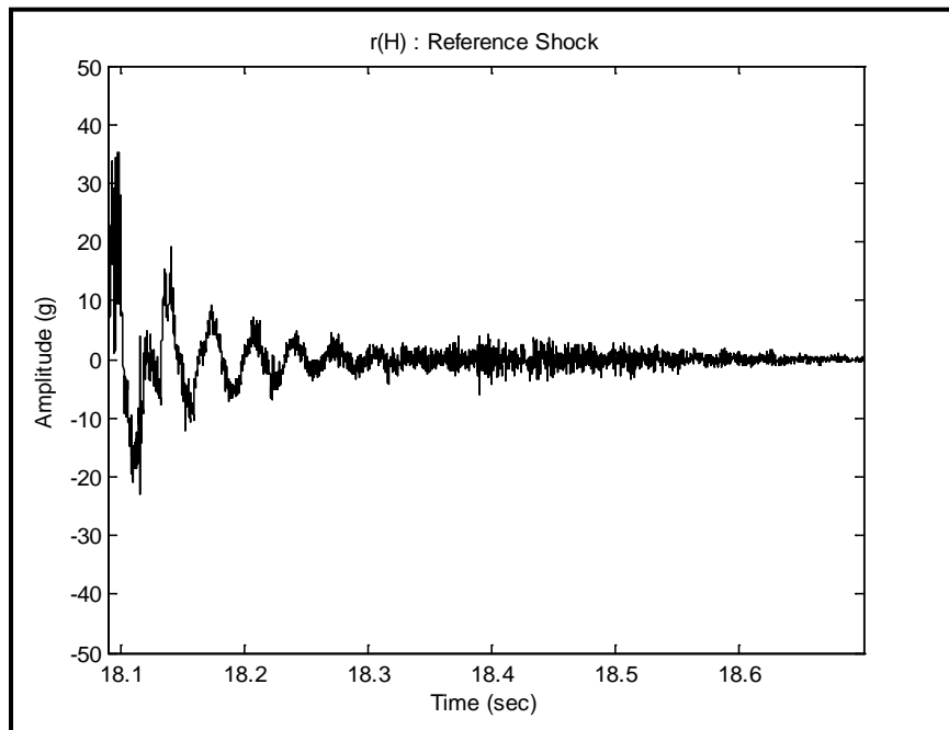
Figure 525.1A-8. Shock reference time trace segment.
