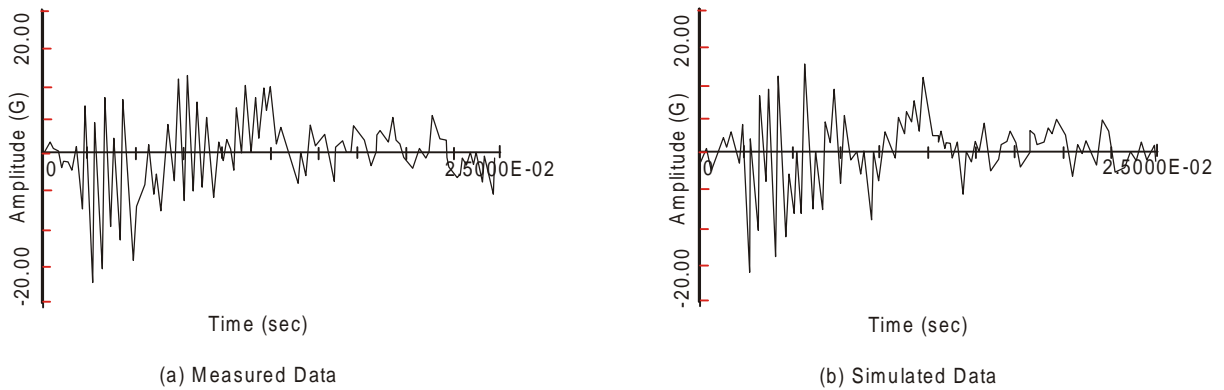
FIGURE 519.5B-2. Ensemble sample time history pulse (pulse 37).
