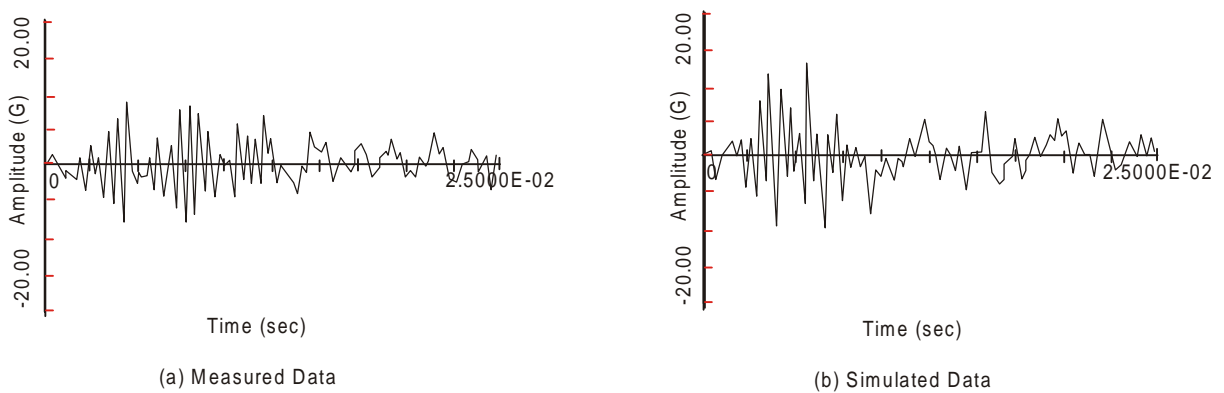
FIGURE 519.5B-3. Ensemble residual sample time history pulse (pulse 37).
