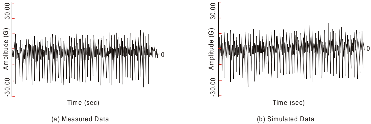
FIGURE 519.5B-1. Fifty round 30mm gunfire event.
